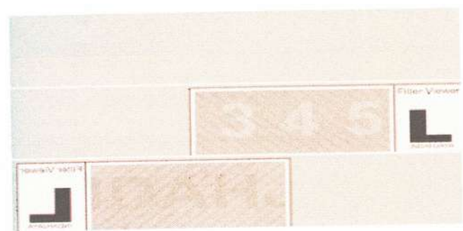
Gambar 4. Filter Image
