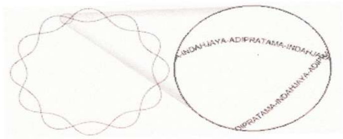
Gambar 6. Microtext
