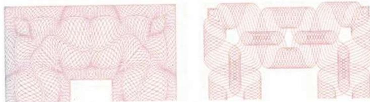
Gambar 3. Guilloche
